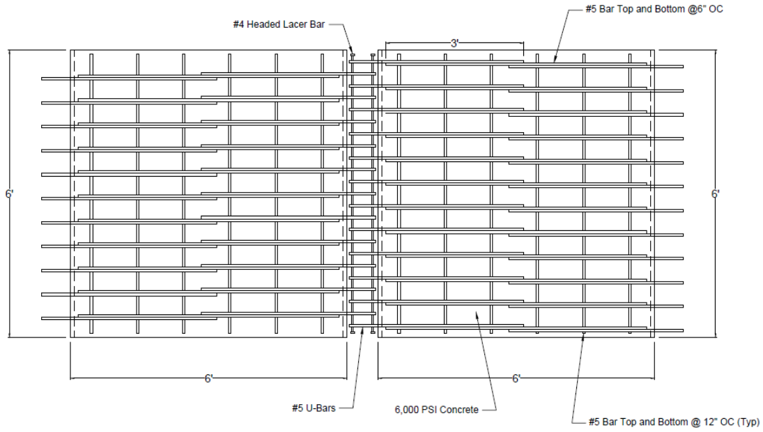
Figure 3.3: Plan view of test specimen
